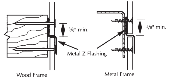
Fig. 5 Horizontal Joints
