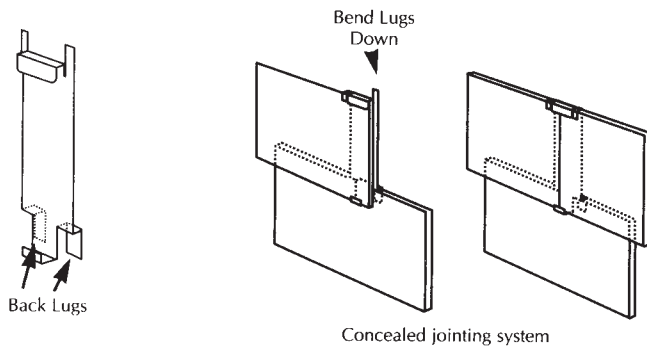
Fig. 11 Metal Joint Plate
