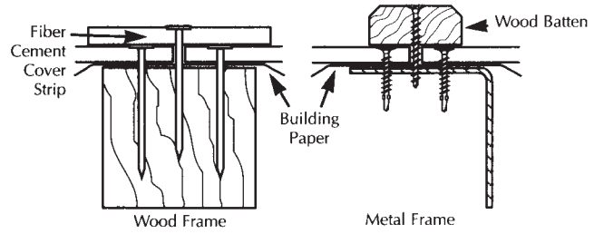
Fig. 4 Vertical Joints
